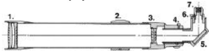
Above: TeleVue 4 inch telescope optical arrangement.
