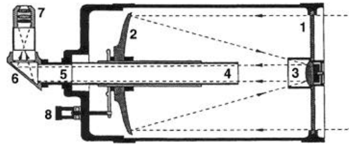
Above: Schmidt-Cassegrain optical arrangement.
